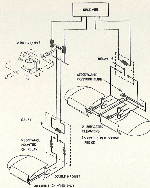
AERODYNAMIC "SPOILER TYPE" CONTROL DIAGRAM FOR Hs. 293 TYPE 1
